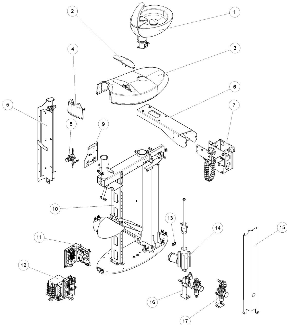
KOSTRA CHEESE L KOMPLET - M11711002101
