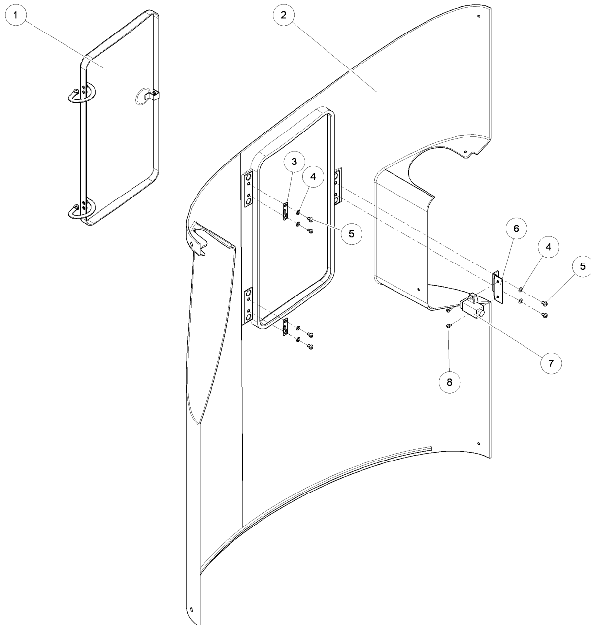
KRYT BP LAVY CHEESE L - M12827002101
