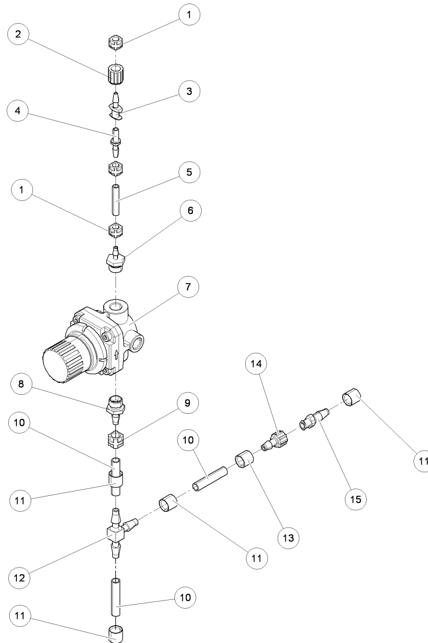
REGULATOR AIR KOMPL.CHEESE L - M13890002301
