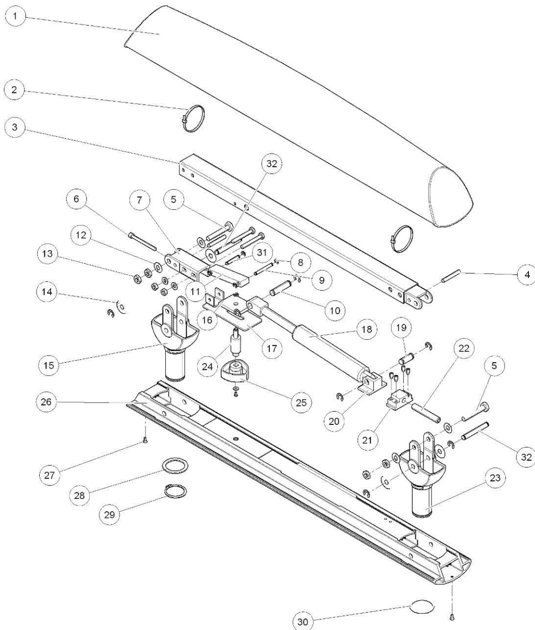
PANTOGRAF STOLIKA- MANUAL (1700) - C11683002103
