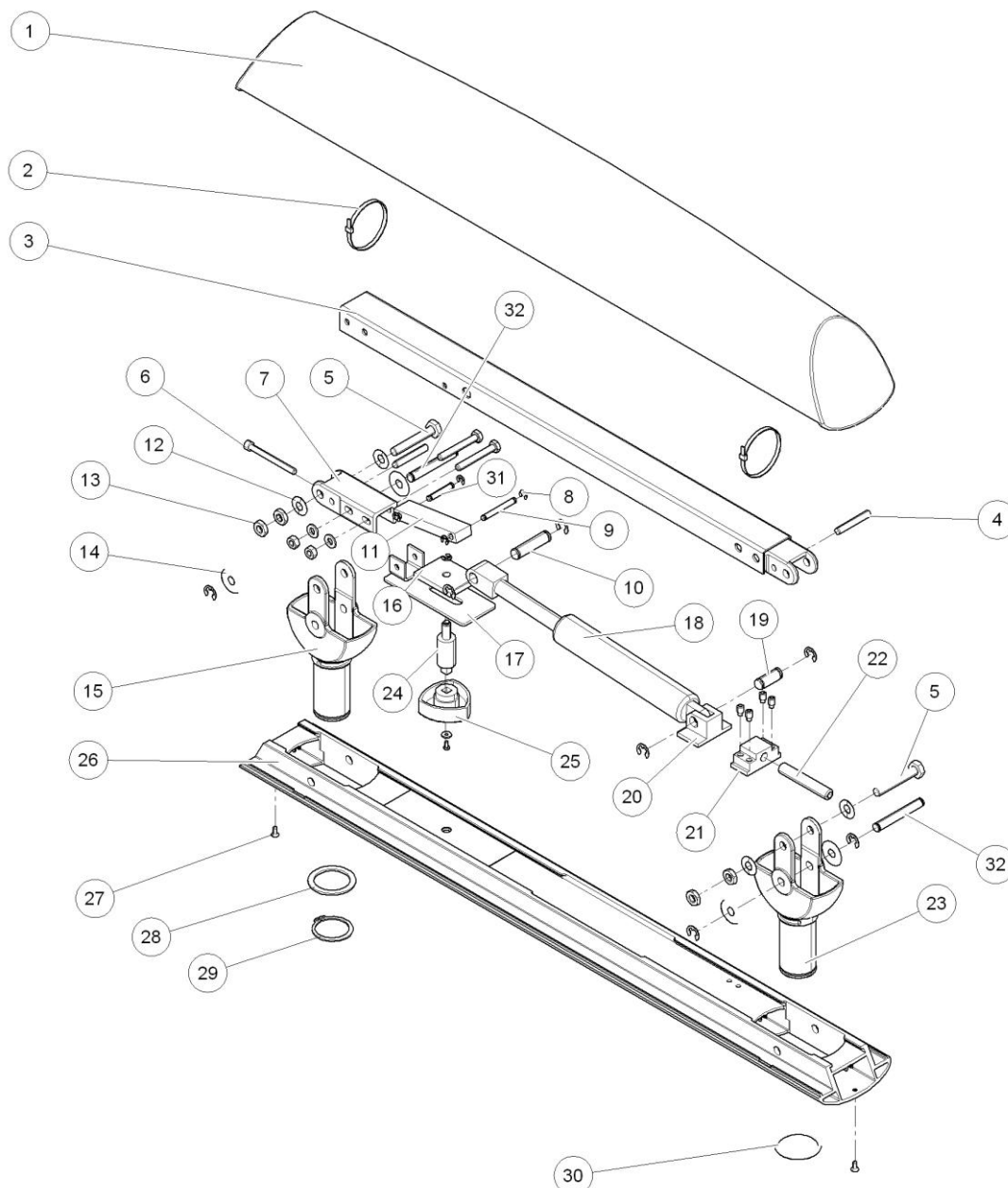
PANTOGRAF STOLIKA- MANUAL (2200) - C08124002104 for dentist table 6N, side keyboard
