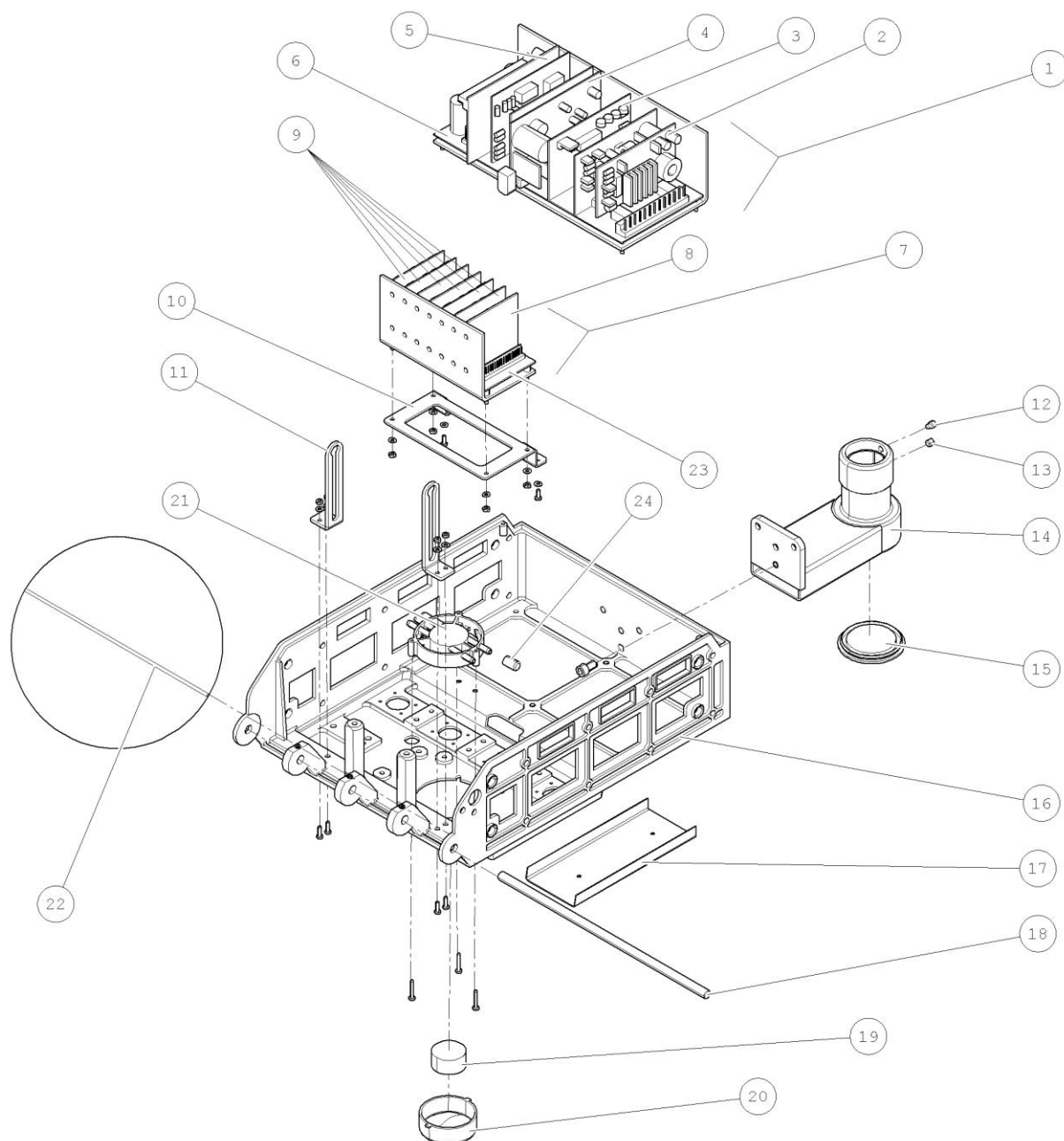
CAST SPODNA 4N-HV-BOCNE OVL.-P - E09290002201 NEW VERSION SINCE OCTOBER 2012
