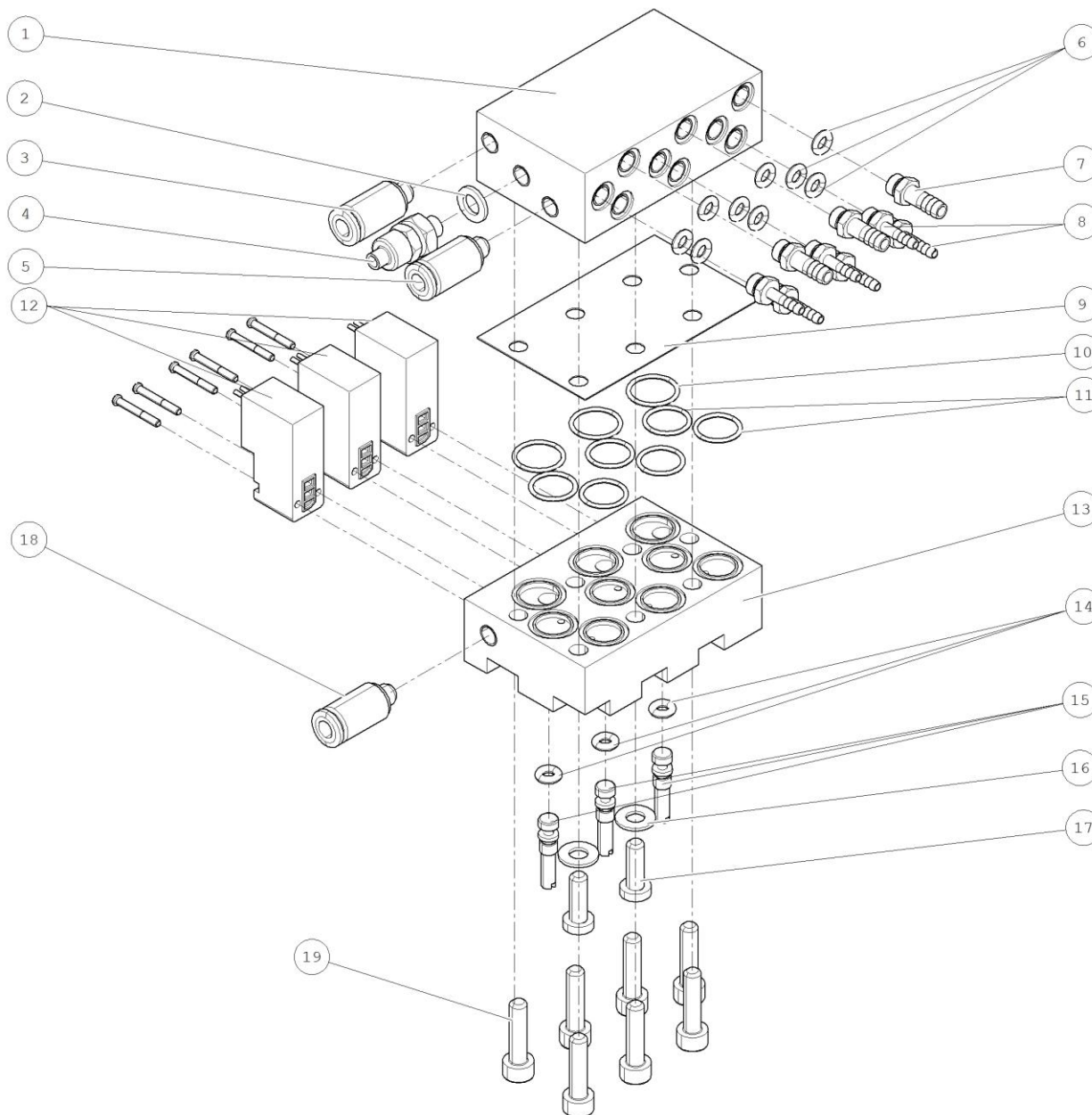
OVLADANIE PNEUMATICKE 3 - J08-11000
