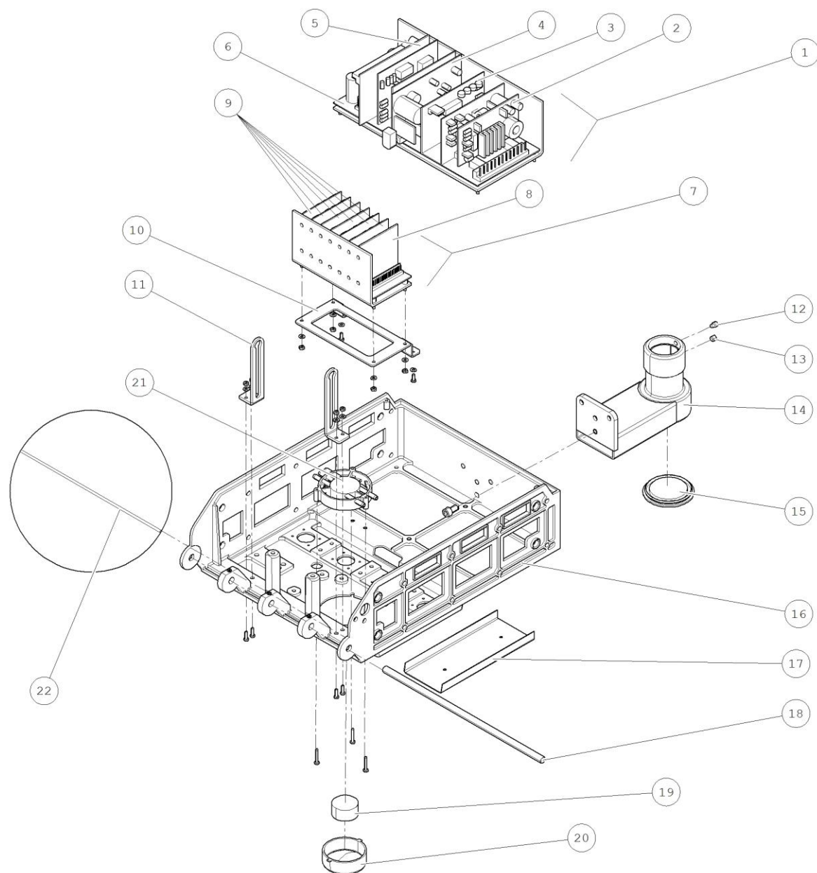
CAST SPODNA 4N-HV-BOCNE OVL.-P - E09290002201
