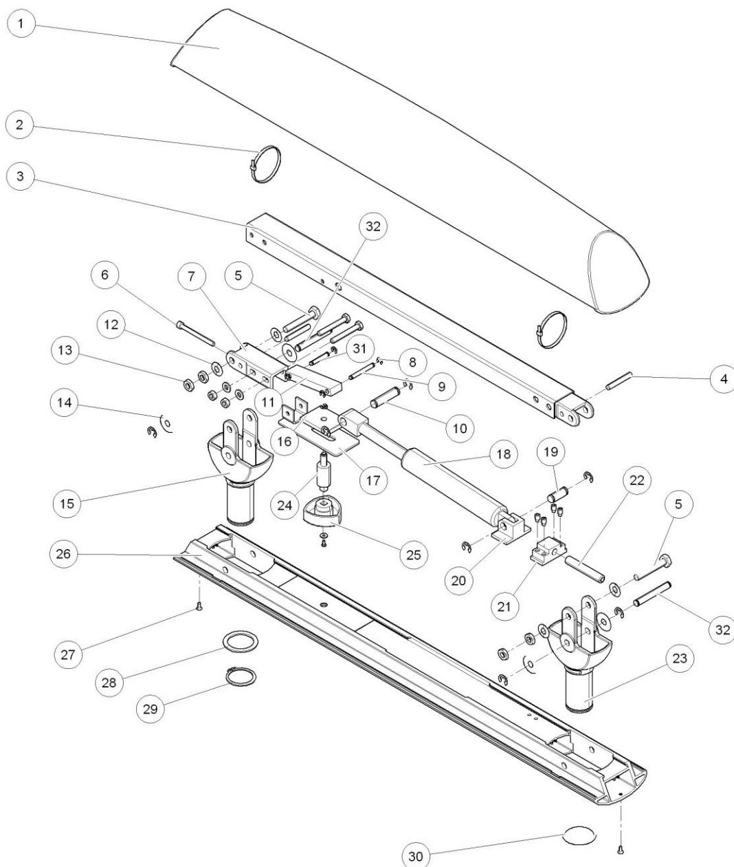
PANTOGRAF STOLIKA - MANUAL (1700) - C08124002105 for dentist table 4N, side keyboard
