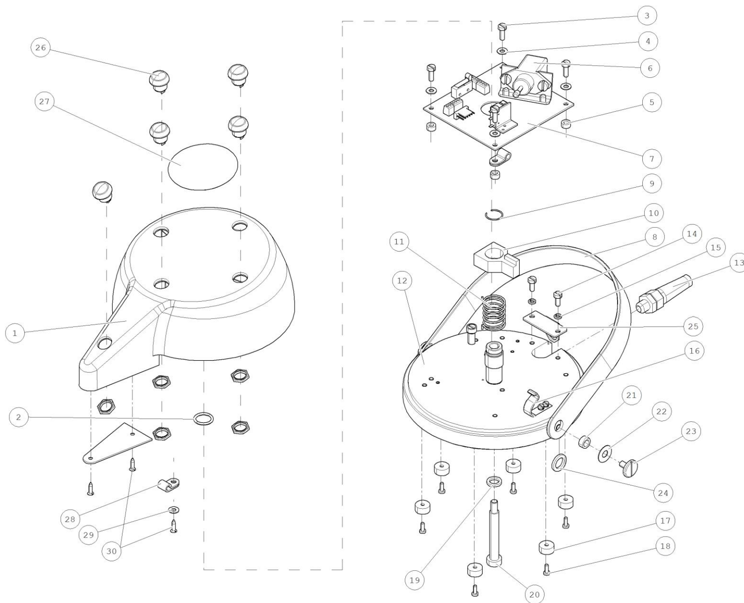
NOZNY OVLADAC MF VELKY – 021294210001
